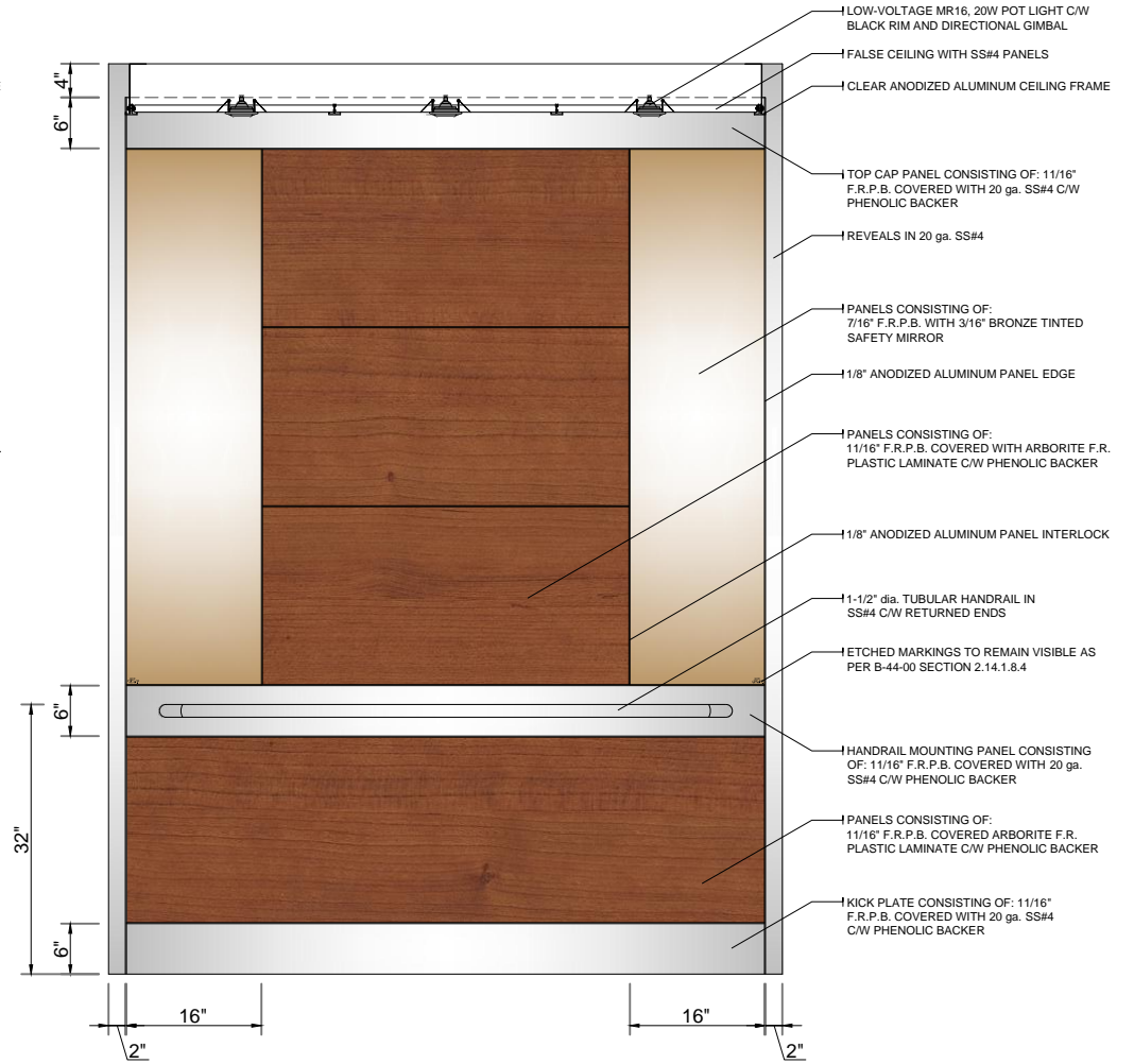
B REAR WALL ELEVATION 1 TYPICAL
