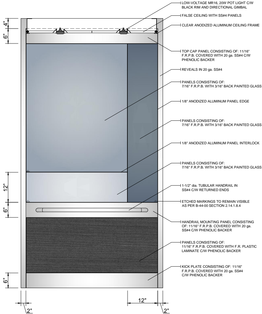
A SIDE WALL ELEVATION 1 TYPICAL
